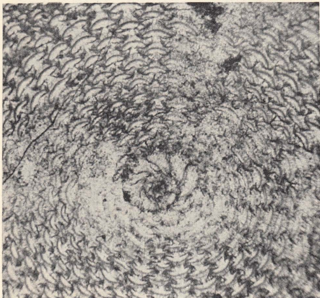
Cole: Helicostegina , Helicolepidina , Lepidocyclina ( Polylepidina )
