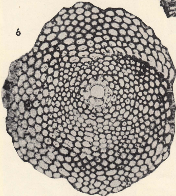
Cole: Helicostegina , Helicolepidina , Lepidocyclina ( Polylepidina )
