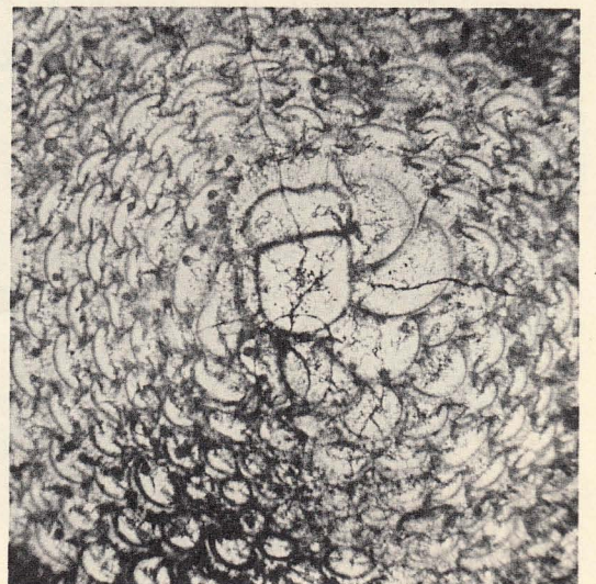
Cole: Helicostegina , Helicolepidina , Lepidocyclina ( Polylepidina )
