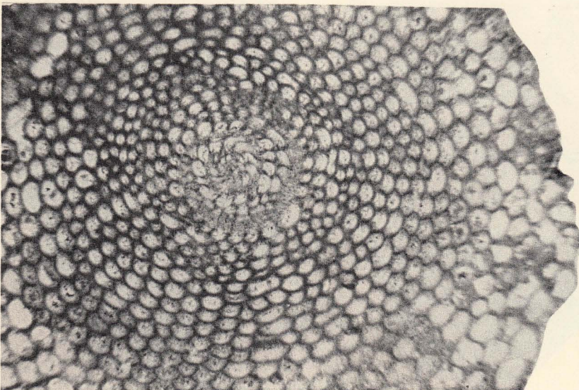
Cole: Helicostegina , Helicolepidina , Lepidocyclina ( Polylepidina )
